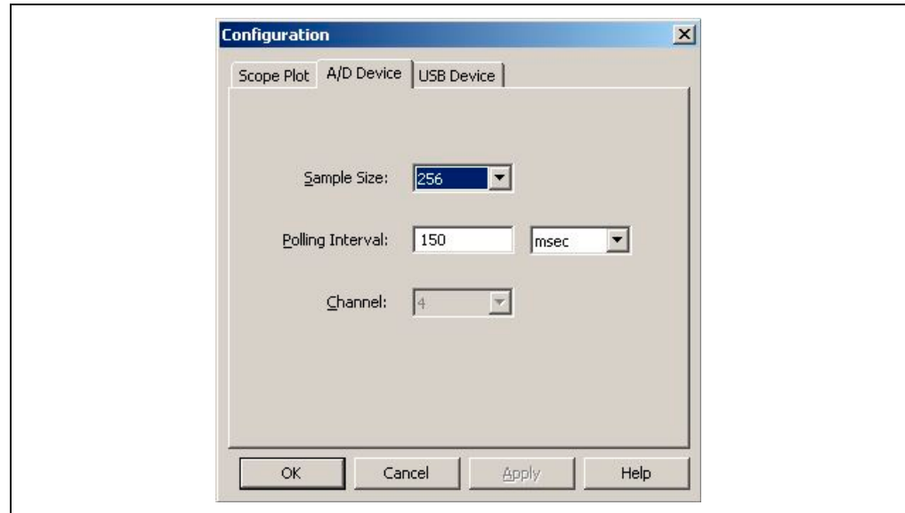
FIGURE 4-4: Configuration Window.
