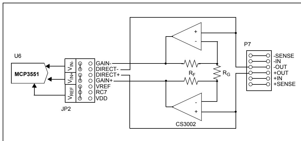
FIGURE 2-5: High Gain Circuit Using CS3002.
