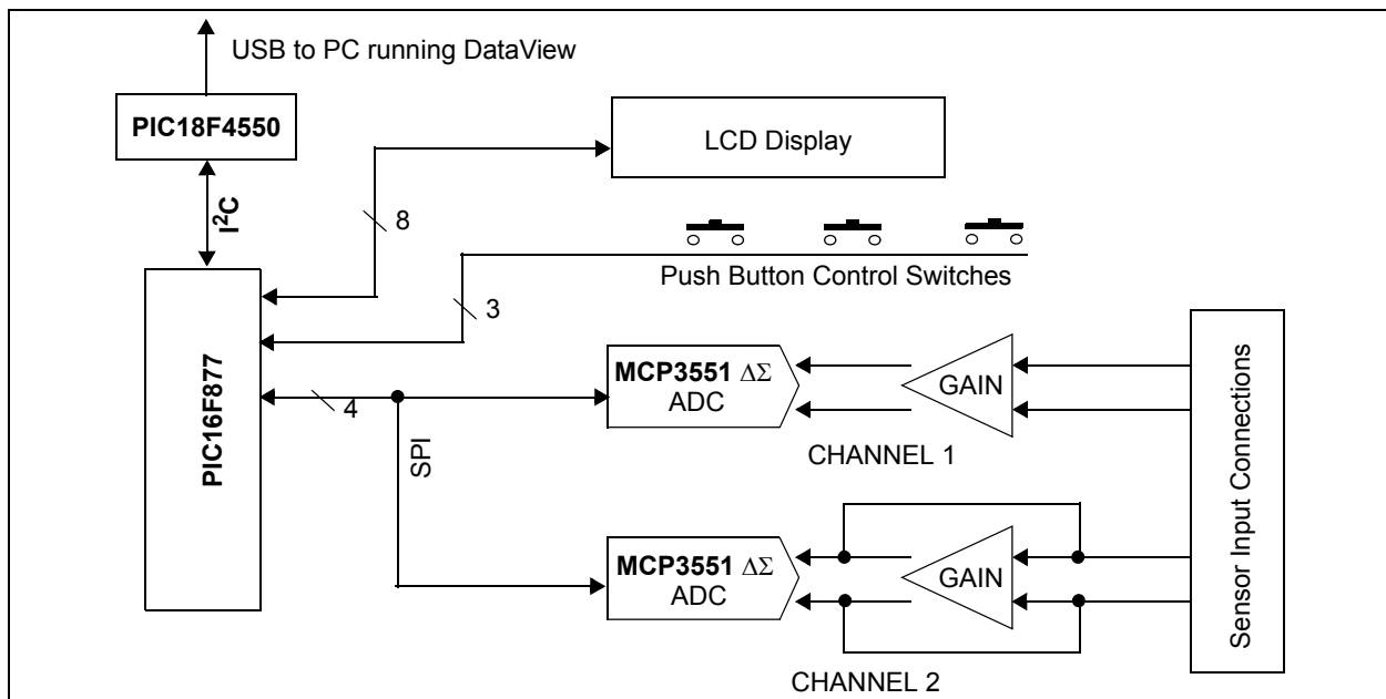
FIGURE 2-1: MCP355X Sensor Application Developer's Board Functional Block Diagram and Results.
