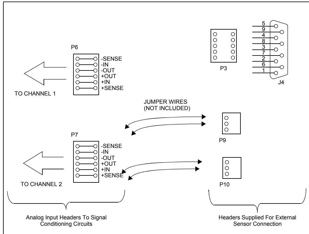
FIGURE 2-2: Sensor Input Connections.
